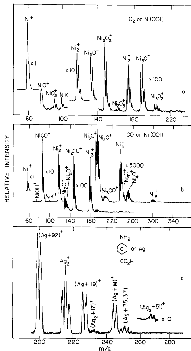
Figure 7. Experimental SIMS spectra. (a) Positive ion spectrum for Ni(001) exposed to 30 L of oxygen. (b) Positive ion spectrum for Ni(001) exposed to 2 L of CO. (c) Positive ion spectrum for p -aminobenzoic acid adsorbed on polycrystalline Ag.
