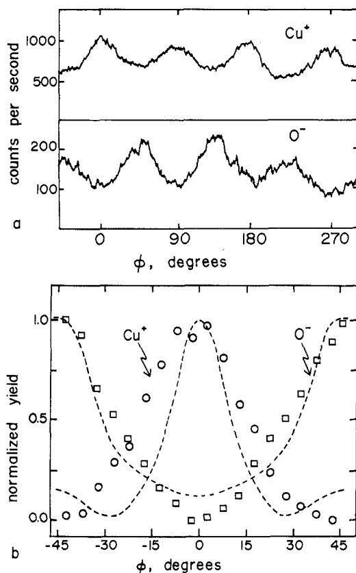
Figure 6. Azimuthal angular distributions. (a) The \text{Cu}^+ and \text{O}^- azimuthal plots recorded from the spectrometer. The primary ion is 1500-eV \text{Ar}^+ at a total dose of 10^{13} ions/cm 2 . (b) A fourfold average of the data in (a) with the minimum intensity subtracted from each curve. The dashed lines represent the calculated curve for O placed in a fourfold bridge site 1.2 Å above the Cu plane. The circles represent the \text{Cu}^+ intensities and the squares the \text{O}^- intensity.
